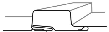
SIDE LAPPING JOIN:
